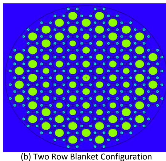
Figure 3.11. Cross Section of Core Configurations Used in Leakage Studies
