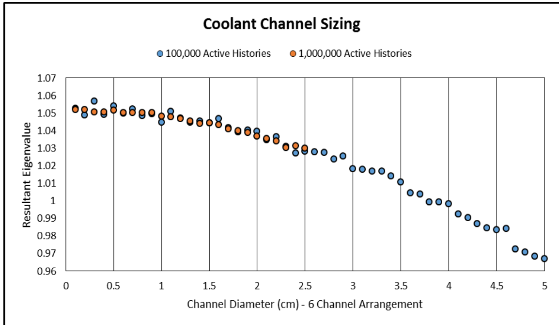
Figure 3.5. Resultant Eigenvalues of Varying Coolant Channel Sizes
